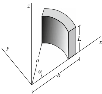
Figure 4.22: The segment of a cylinder with uniform charge density used in Problem 4.41.
