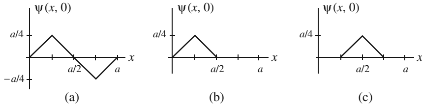
Figure 28.1: The initial shape of the waves.
