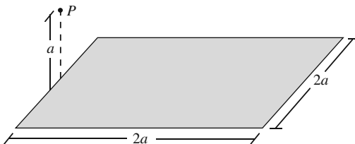
Figure 4.19: The figure for Problem 4.28.
