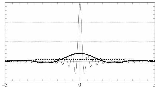
Figure 18.7: The function \sin Tx/x also approaches the Dirac delta function as the width of the curve approaches zero. The value of T is 0.5 for the dashed curve, 2 for the heavy curve, and 15 for the light curve.
