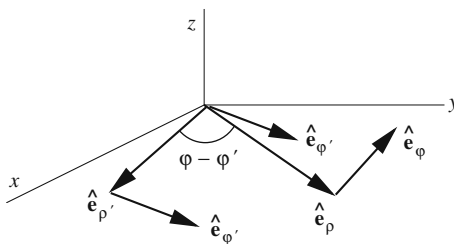
Figure 4.7: The orientation of some of the cylindrical unit vectors drawn for the calculation of cross products.
