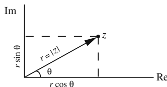
Figure 18.3: Complex numbers in polar coordinates.
