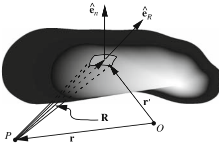
Figure 12.4: Solid angle as the ratio of area to distance squared.
