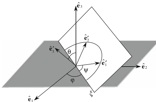
Figure 6.7: The Euler angles and the rotations about three axes making up a general rotation in space.
